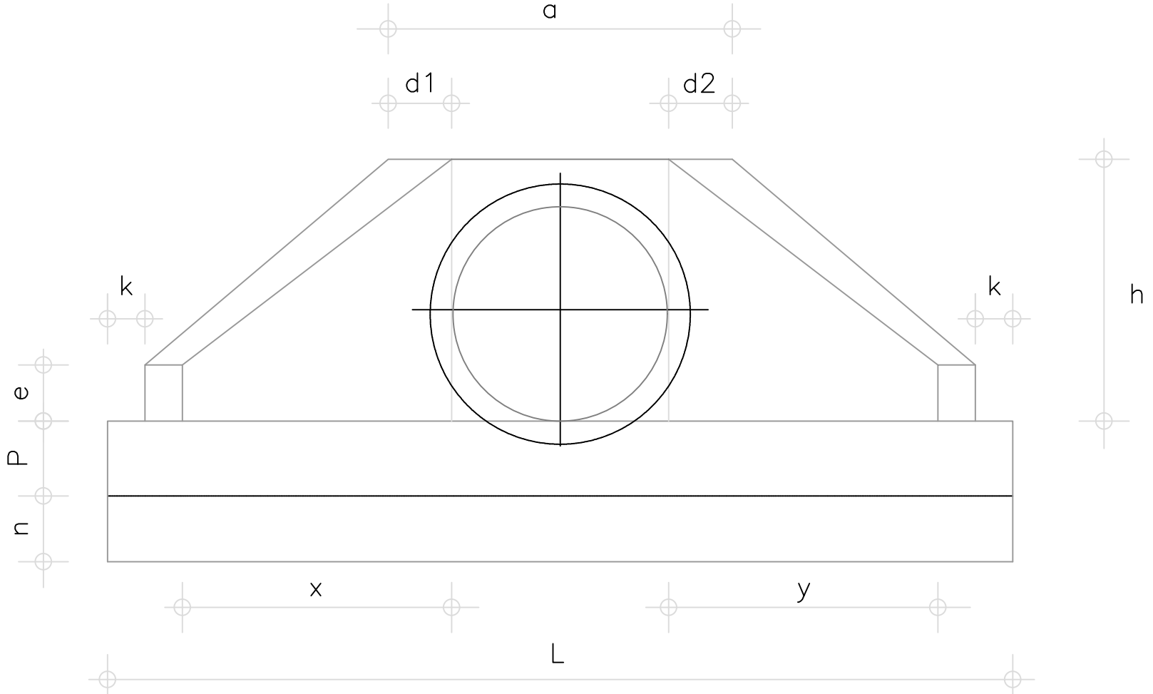
VISTA FRONTAL
